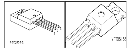
PG-TO220-3-31 PG-TO220
